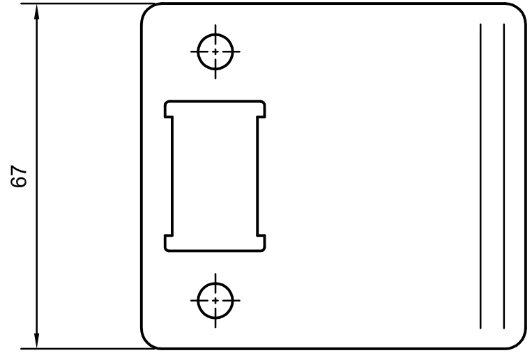
EXTENDED STRIKE PLATE (SINGLE DOORS) 5245 ESP
