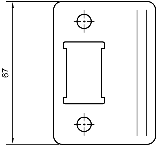
STANDARD STRIKE PLATE (DOUBLE DOORS) 5235
